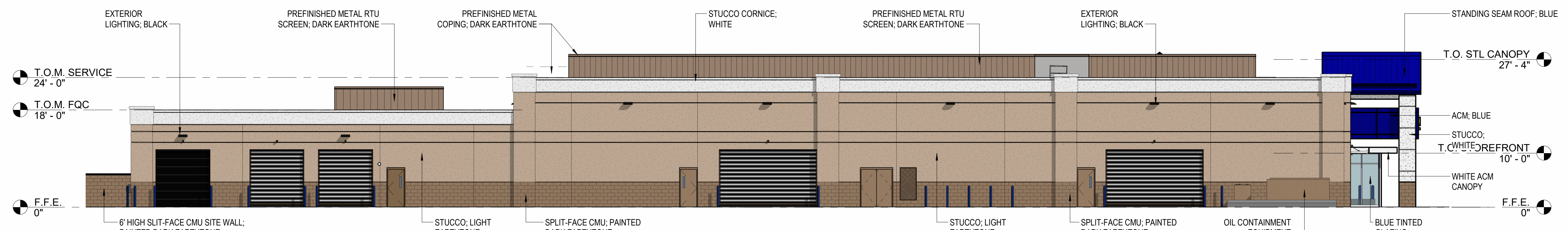
4 WEST ELEVATION A 3.0 3/32" = 1'-0"
